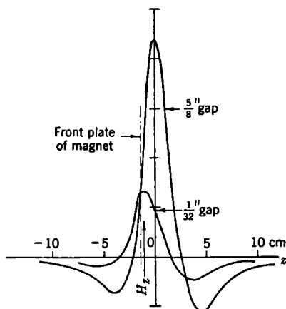
FIG. 3-18.—Intensity of the axial component H_z of the focus field along the axis for the focus magnet shown in Fig. 3-17.
